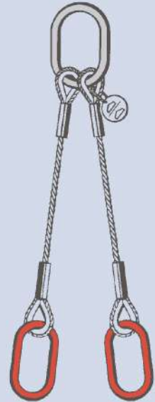
1226. 2-leg wire rope sling with master links
