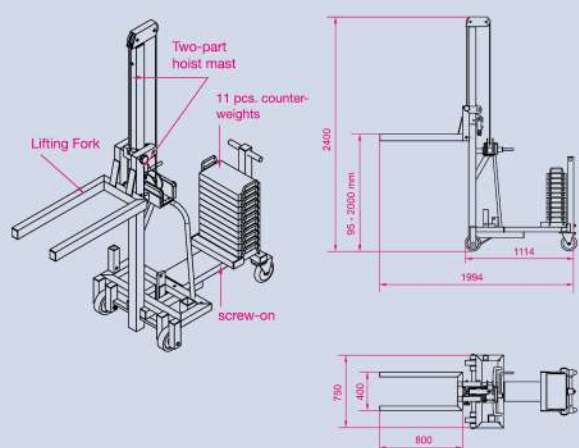
Figure 4 with counterweight, with lifting fork
