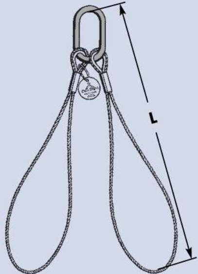
1230 2-leg wire rope sling consisting of 1 master link & 2 wire rope loops
