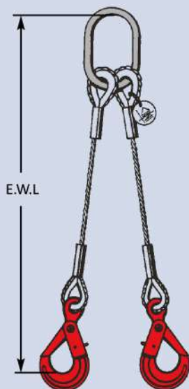
1217. 2-leg wire rope sling with self-locking eye hook
