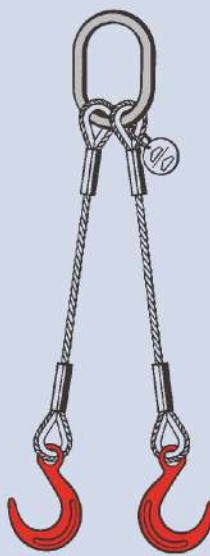
1218. 2-leg wire rope sling with foundry hook
